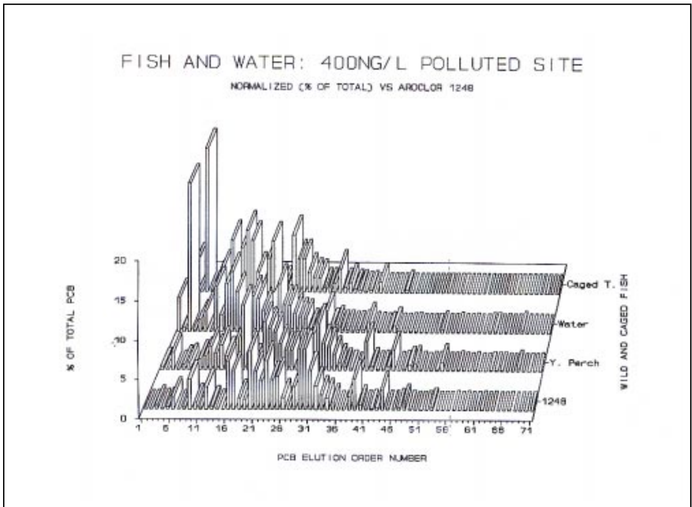
Figure 4. Comparison of PCB patterns in caged trout, wild fish (yellow perch) and water from Contaminant Cove, Akwesasne on the St. Lawrence River and Aroclor 1248.
