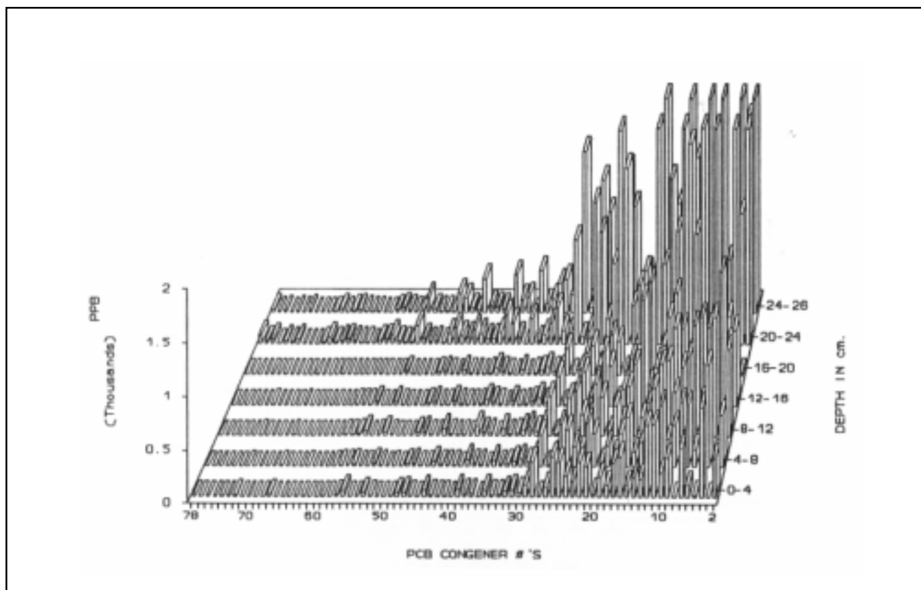
Figure 1. PCB congener patterns from a 26 cm core taken at Grif-fin Island in the upper Hudson River.
