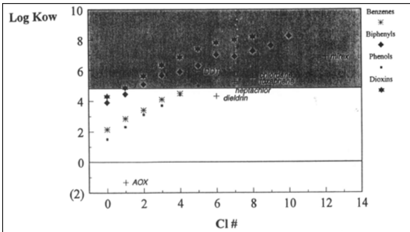
Figure 2. Plot of KOW versus chlorine number for various homologous series of organic compounds showing that addition of sufficient chlorines causes substances to achieve a level hydrophobicity (log KOW of 5) sufficient to cause appreciable bioconcentration, as indicated by the shaded zone (adapted from Mackay and DiGuardo 1994).
