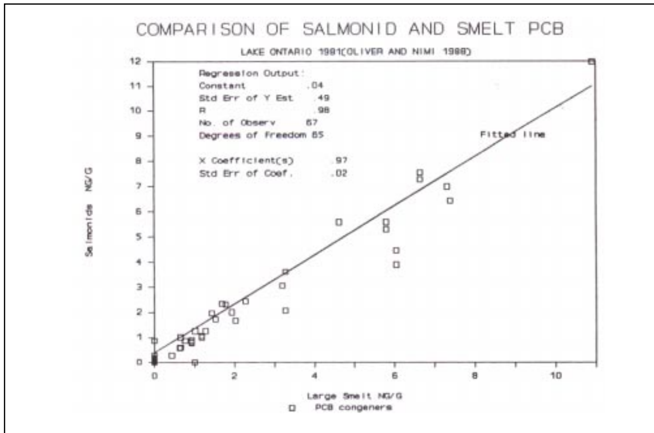
Figure 3. Comparison of the PCB congener concentrations in large smelt and salmonids reported by Oliver and Nimi (1988) from Lake Ontario in 1981 .
