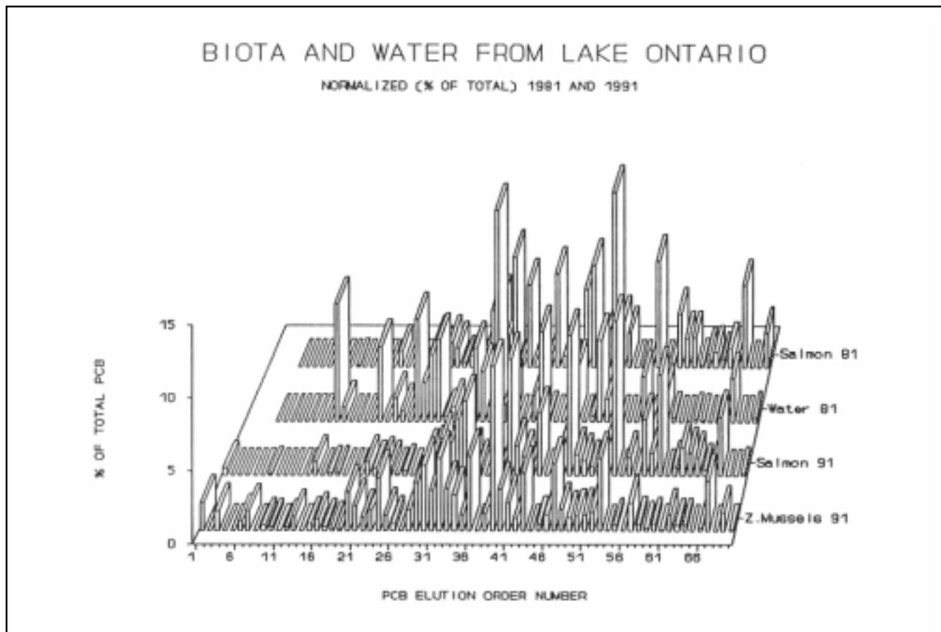
Figure 2. Patterns of PCB pollution from Lake Ontario. 1981 data are from Oliver and Nimi (1988) reordered to match data from this laboratory.
